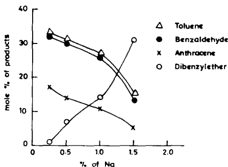
FIG. 2. Effect of sodium ion content of alumina on product distribution.
